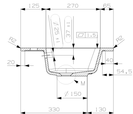
SECTION L-L SCALE 0.143:1.0
