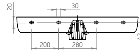
Backside view 1:16
