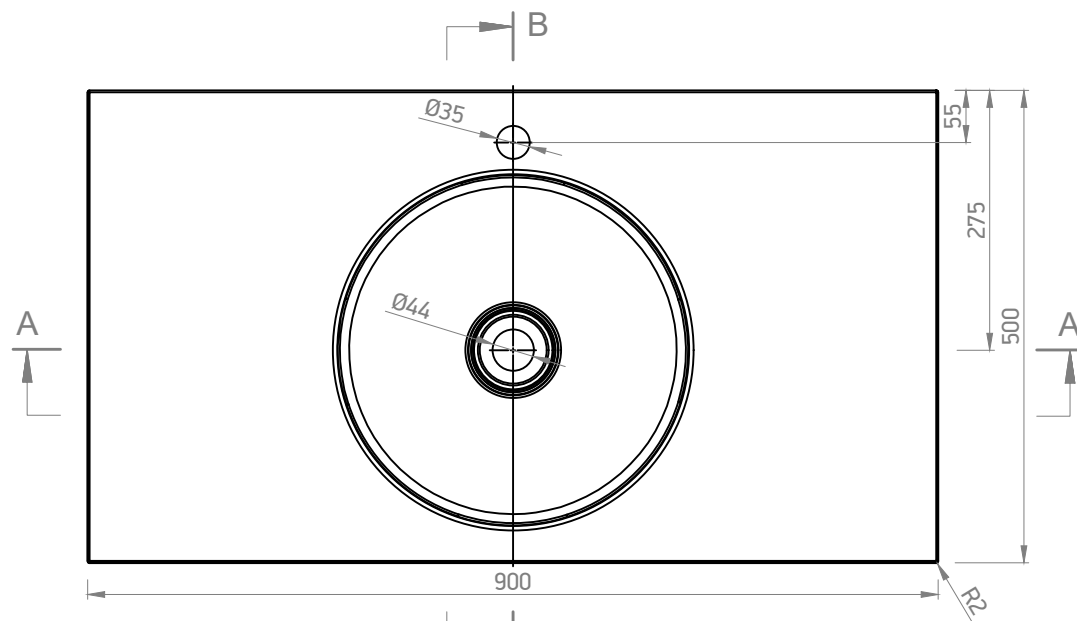
Bottom view 1:16
