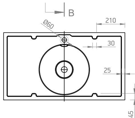
Bottom view 1:16
