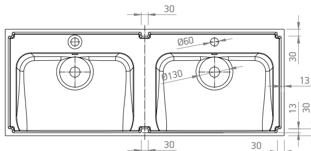
Bottom view 1:16
