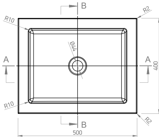
Bottom view 1:16
